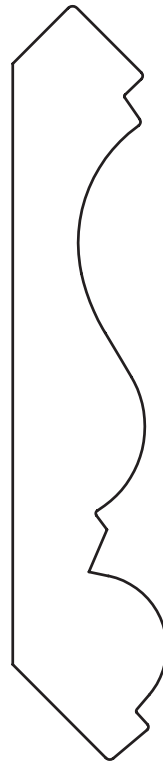
13/16" x 3-15/16" Crown
