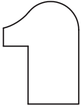
3/4" x 1-1/16" Back Band 5/8" rabt
