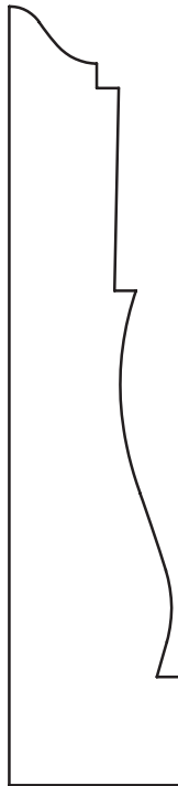
13/16" x 3-11/16" Casing JMC 4344
