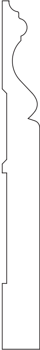
1 1/16" x 6-1/4" Base
