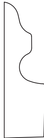
3/4" x 2-1/2" Casing
