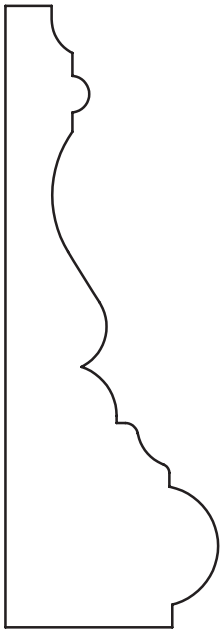
1-1/8" x 3-1/4" Casing
