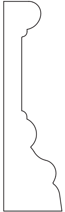
1" x 3-1/2" Casing
