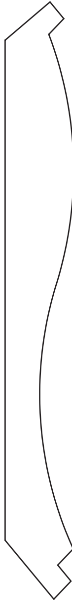
3/4" x 6-1/4" Crown
