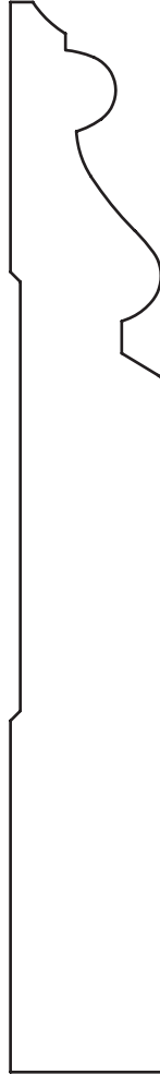
3/4" x 5-1/8" Base
