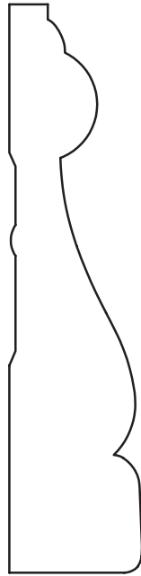
3/4" x 3-5/16" Casing
