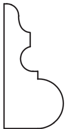
5/8" x 1-5/16" Panel Mould
