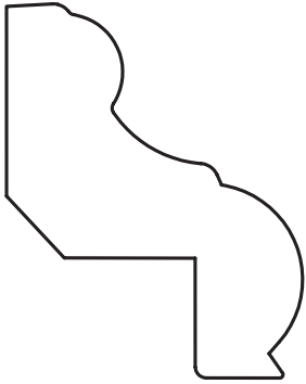
13/16" x 1-13/16" Panel Mould 3/4" rabt
