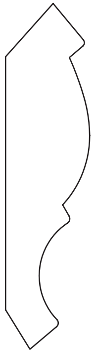
7/8" x 3-5/8" Crown
