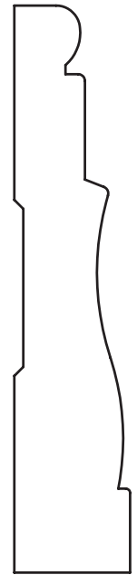
11/16" x 3-1/4" Casing
