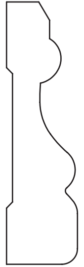
3/4" x 2-3/4" Casing
