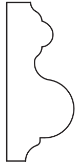
11/16" x 1-5/8" Panel Mould
