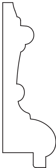
7/8" x 2-3/4" Panel Mould 5/8" rabt
