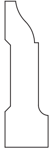
3/4" x 2-1/2" Casing
