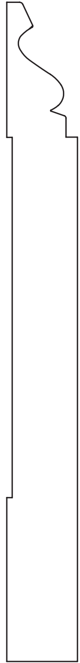
3/4" x 7" Base
