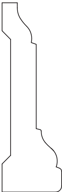
1" x 3-3/8" Casing
