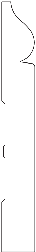
11/16" x 5-3/16" Base
