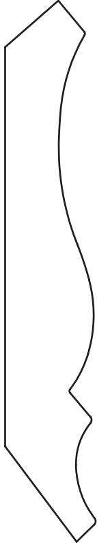
3/4" x 4-1/8" Crown
