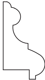
13/16" x 1-5/16" Panel Mould 1/2" rabt
