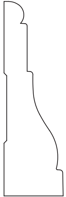
1" x 3-3/8" Casing
