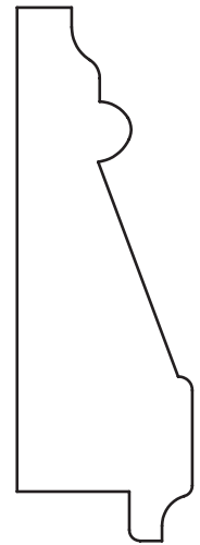
7/8" x 2-5/8" Panel Mould 5/8" rabt
