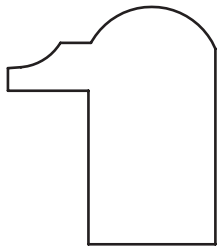
1-1/16" x 1-1/4" Back Band 13/16" rabt
