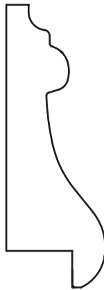
3/4" x 2-1/8" Panel Mould 1/2" rabt
