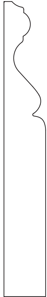
3/4" x 5-5/16" Base
