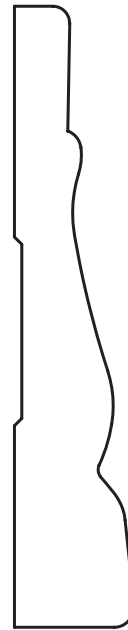
5/8" x 3-1/4" Casing
