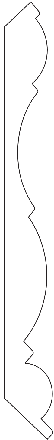
13/16" x 7-1/2" Crown
