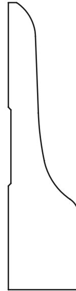
3/4" x 2-15/16" Casing
