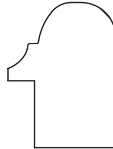
1-1/16" x 1-1/2" Back Band 3/4" rabt
