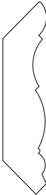
3/4" x 3-1/4" Crown
