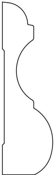
7/8" x 2-15/16" Chair Rail
