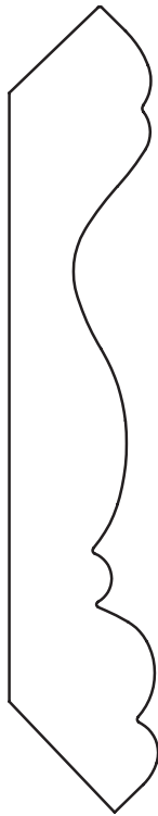
11/16" x 3-7/8" Crown
