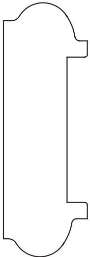
1-1/16" x 2-11/16" Shoe Rail
