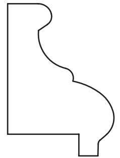
1-1/8" x 1-5/8" Panel Mould 3/4" rabt
