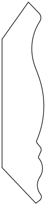
3/4" x 3-9/16" Crown
