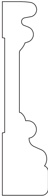
1" x 4-3/16" Casing
