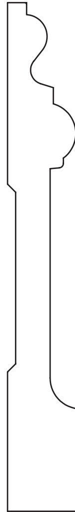
3/4" x 5-5/16" Base
