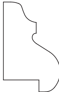
1-3/16" x 1-9/16" Panel Mould 13/16" rabt
