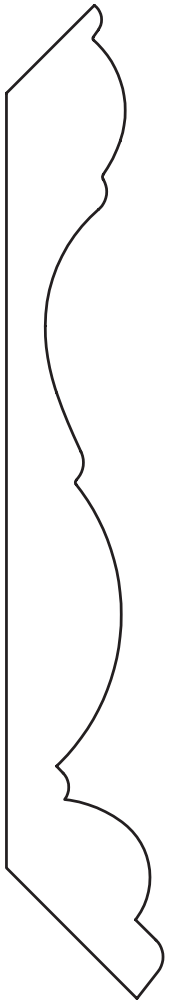
13/16" x 5-3/16" Crown
