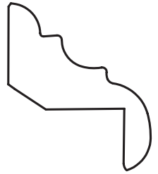
1/2" x 1-1/4" Panel Mould 3/4" rabt
