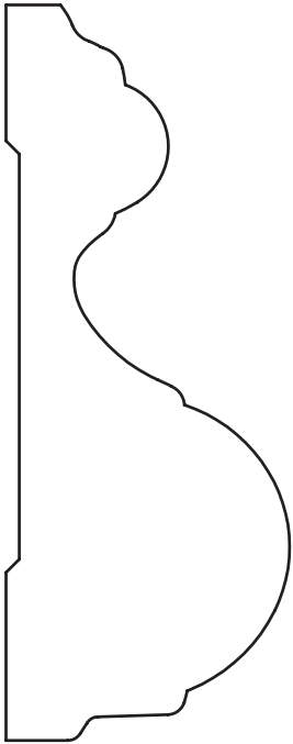
1-3/8" x 3-1/2" Mantel Mould
