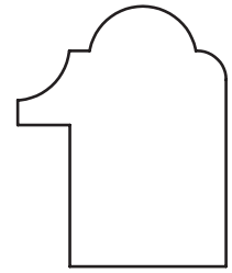
1-1/16" x 1-1/4" Back Band 11/16" rabt
