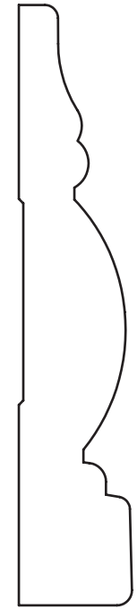
3/4" x 3-1/2" Casing
