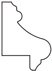
7/8" x 1-1/4" Panel Mould 1/2" rabt
