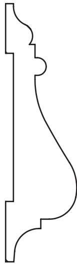
3/4" x 2-11/16" Chair Rail
