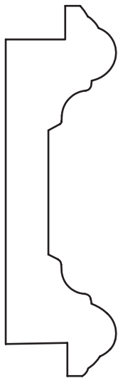
13/16" x 2-3/4" Panel Mould 1/2" rabt
