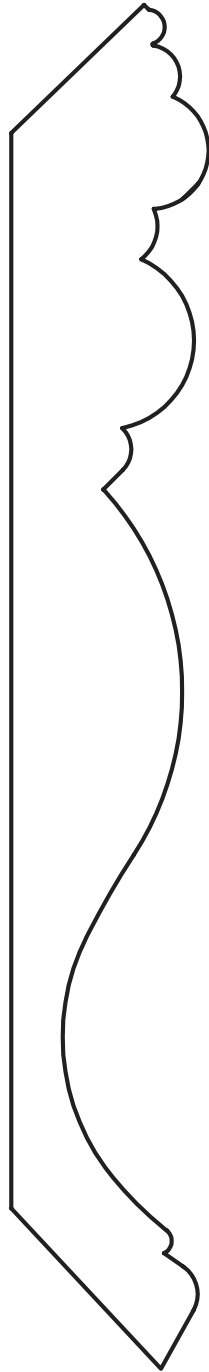
1-1/16" x 7-1/8" Crown
