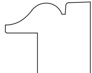
1-5/16" x 1-9/16" Back Band 3/4" rabt
