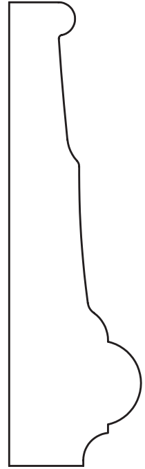
1" x 3-1/2" Chair Rail
