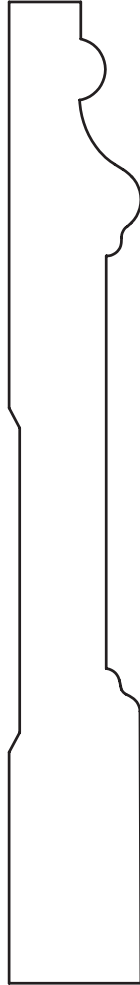
11/16" x 5-1/8" Base
