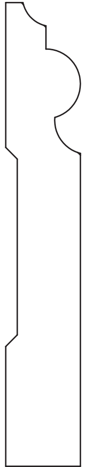
13/16" x 5" Base
