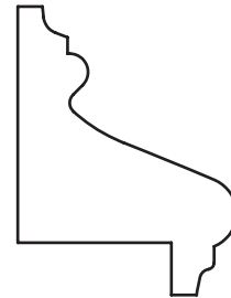
1-1/16" x 1-3/8" Panel Mould 3/4" rabt
