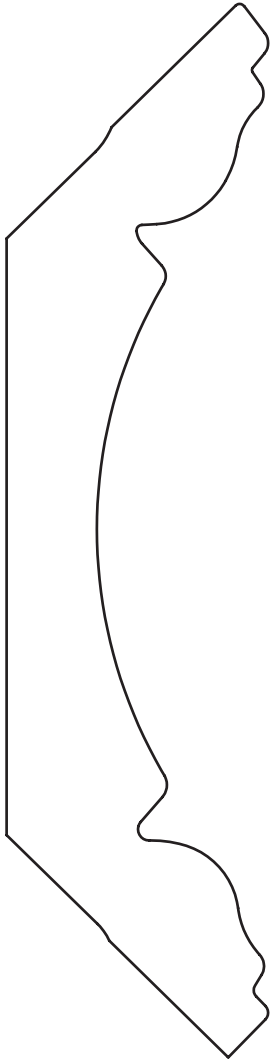
1-1/4" x 5-1/2" Cove Crown
