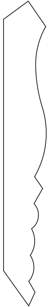
7/8" x 5-1/2" Crown
