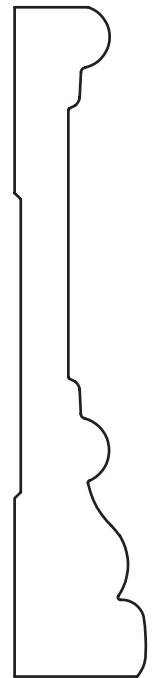
11/16" x 3-1/2" Casing
