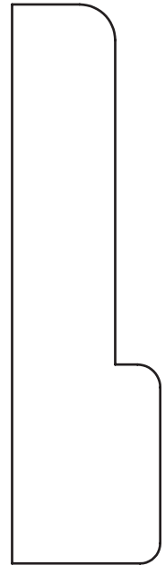
13/16" x 3-1/4" Casing
