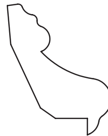
3/4" x 1-5/8" Panel Mould 1/2" rabt
