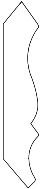
5/8" x 3-1/4" Crown
