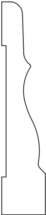
3/4" x 3-5/8" Casing JMC 2388
