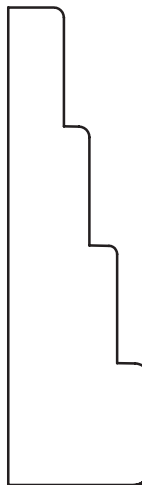
3/4" x 2-1/2" Casing
