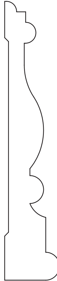
1" x 5" Casing
