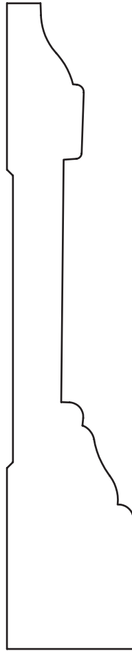
1" x 4-7/8" Casing
