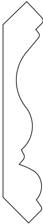
11/16" x 3-3/4" Crown
