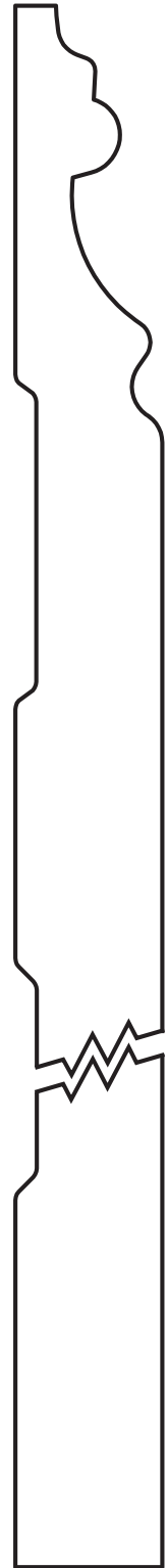
3/4" x 9-1/4" Base
