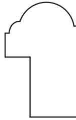
7/8" x 1-3/16" Back Band 3/4" rabt
