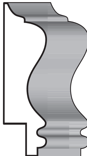
3043 3/4" x 2-5/8" Rab't Chair Rail
