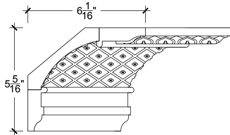
LCD8254 - shows sections & dimensions
