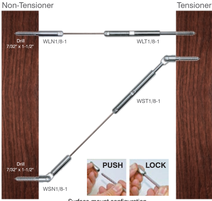
Surface-mount configuration
