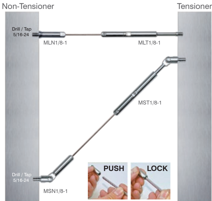
Surface-mount configuration
